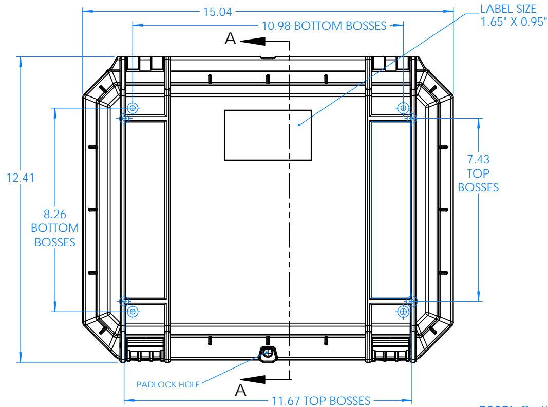
530PL Optional latches with plastic lock
