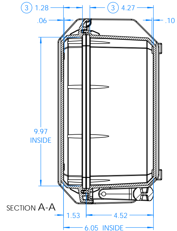
530ML Optional latches with plastic lock
