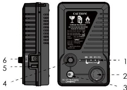
Figure 3: Battery Pack
