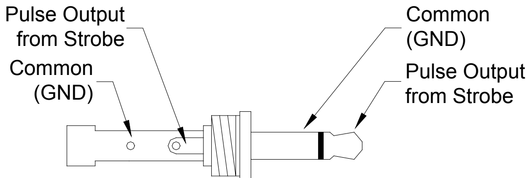
Figure 3 Output Connector Detail (Mono plug)
