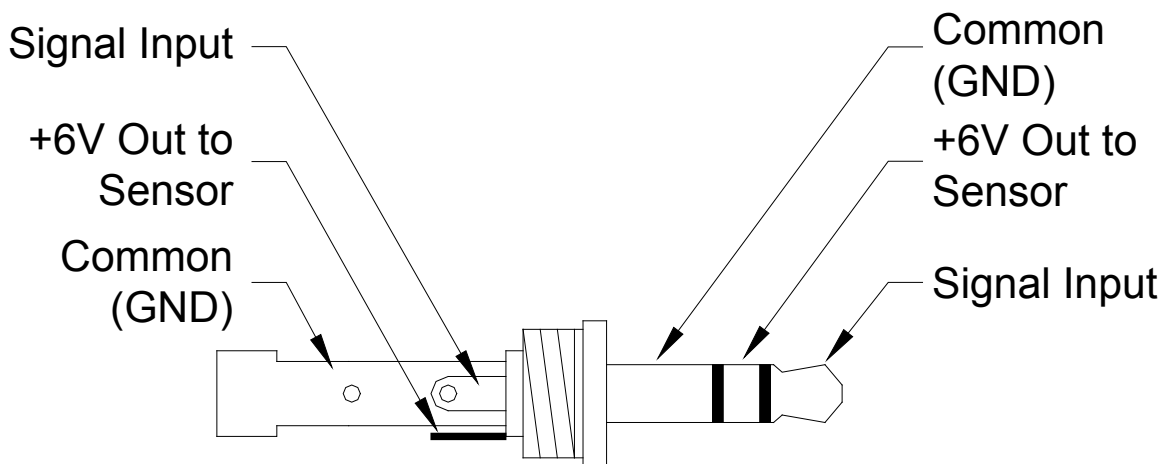
Figure 2 Input Connector Detail (Stereo plug)
