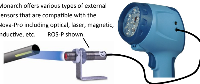
Figure 6 Strobe with External Sensor
