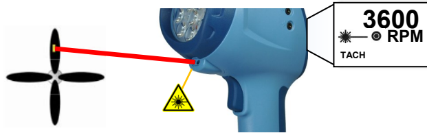
Figure 7 Using the Laser Module
