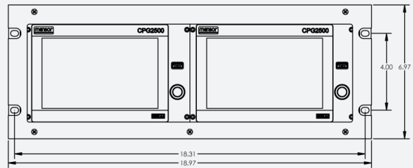
Dual mount - Front view
