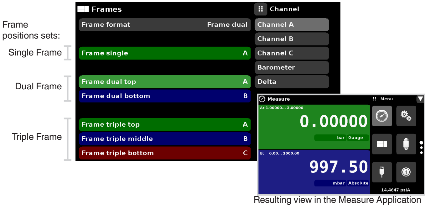
Figure 6.4.3.2 - Frames Channel
