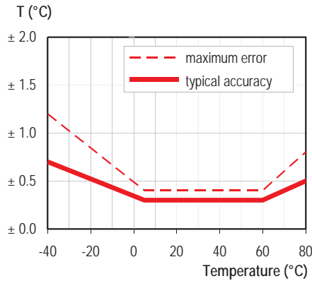
Typical and maximal tolerance for temperature.
