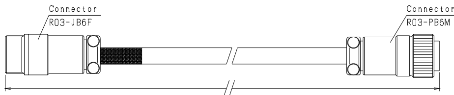
Extension cable(2m~30m)
