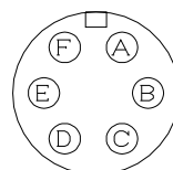
Connector (Soket;R03-PB6M)
