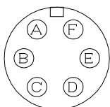
Connector (Pin;R03-JB6F)
