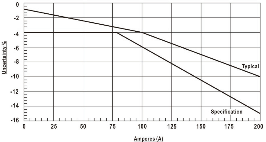
Figure 8: DC signal linearity in the 10 mV/A range, typical
