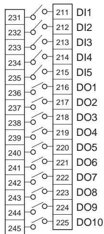
Alarm output/DI input terminal
