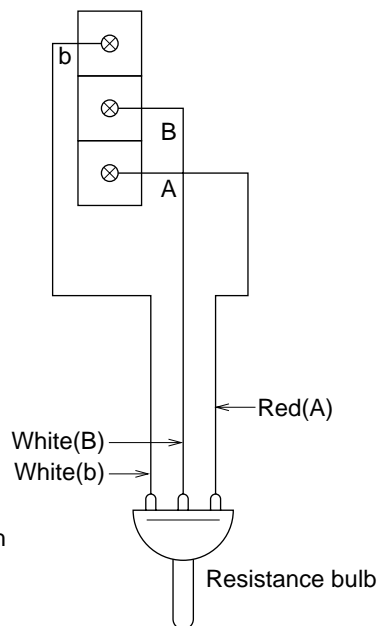
(4) Resistance input
