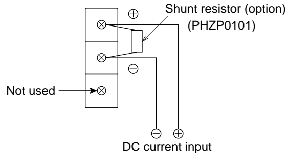
(2) DC current input
