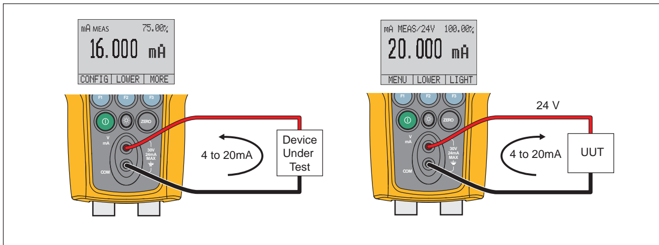
Figure 6. Measure Current
