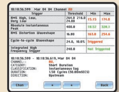
Provides information about the type and severity of the sag and indicates the direction of the sag relative to the monitoring point.
