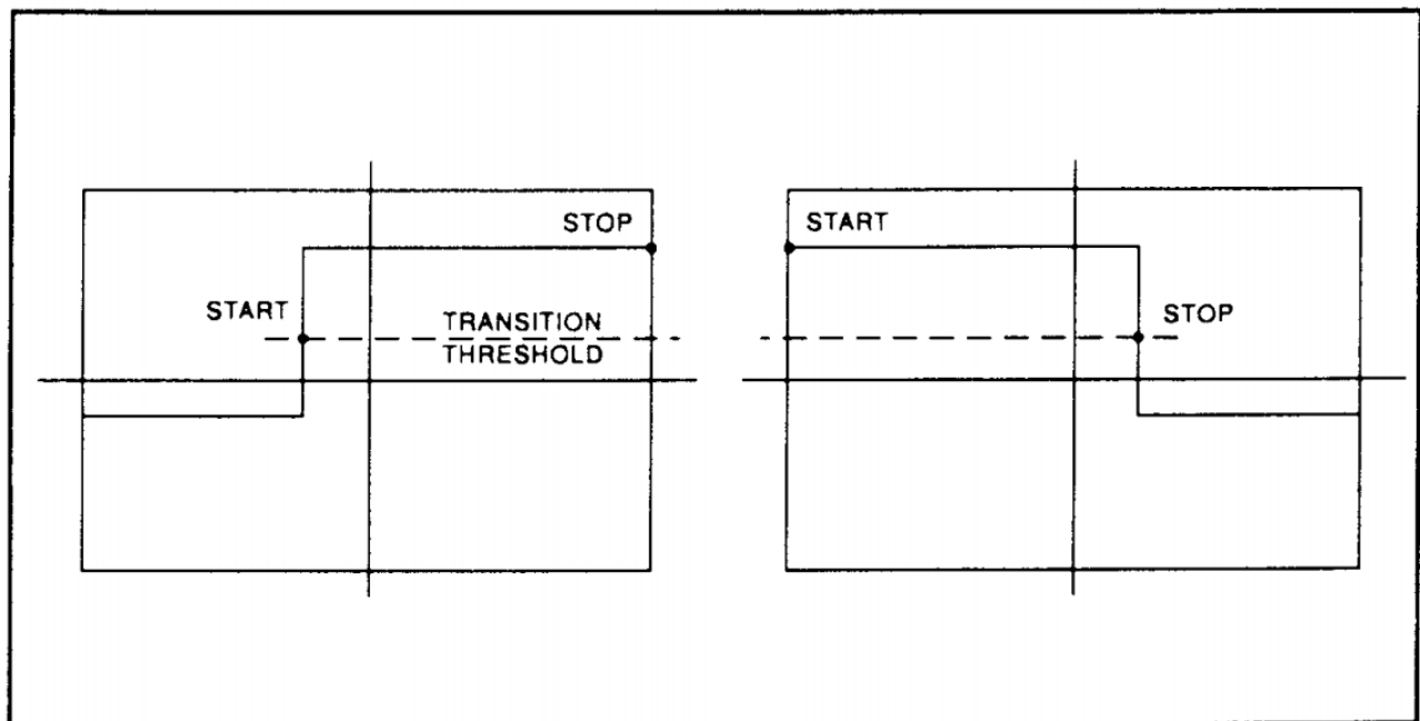
Figure 5.5 Step Waveforms
