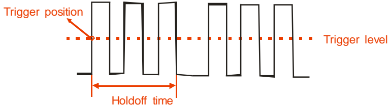
Figure 39 - Trigger Holdoff
