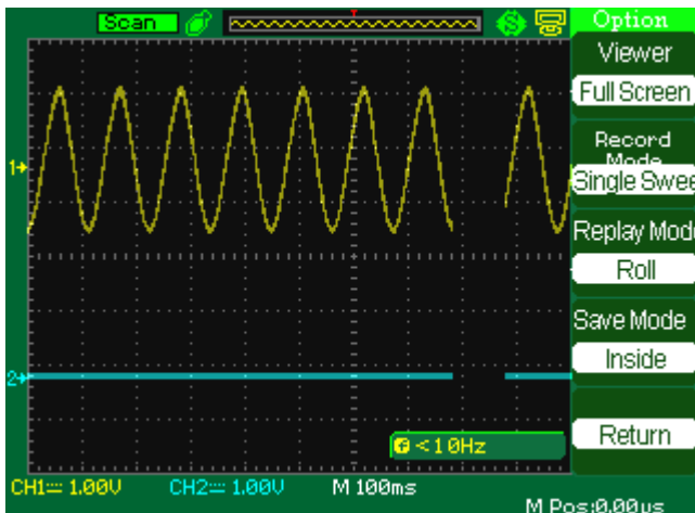
Figure 85 - Option Screen
