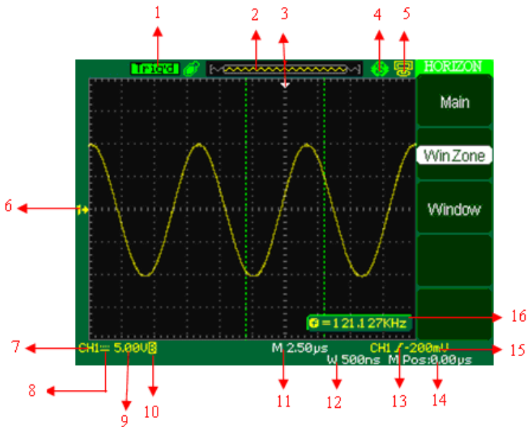
Figure 4 - Display Screen
