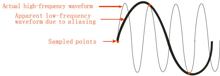
Figure 43 - Time Domain Aliasing
