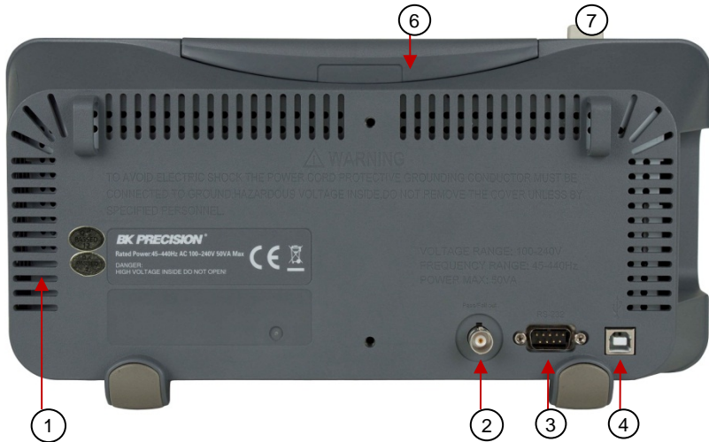
Figure 2 - Back Panel
