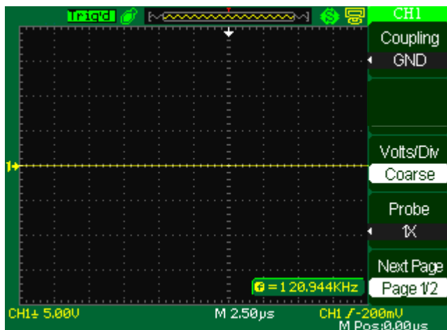
Figure 17 - GND Coupling
