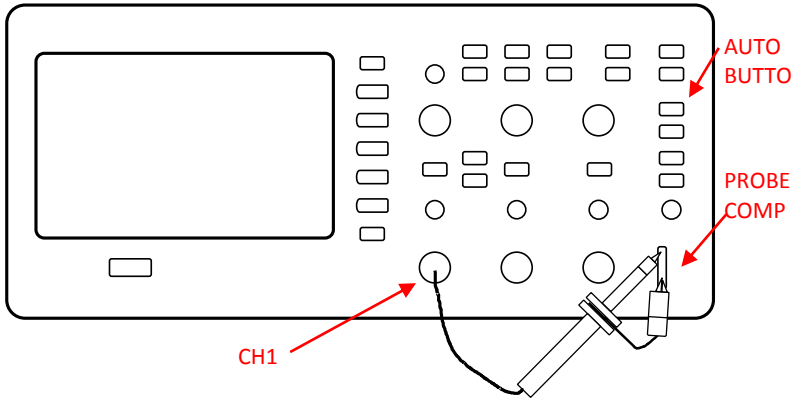
Figure 2.6 – Probe Compensation Setup
